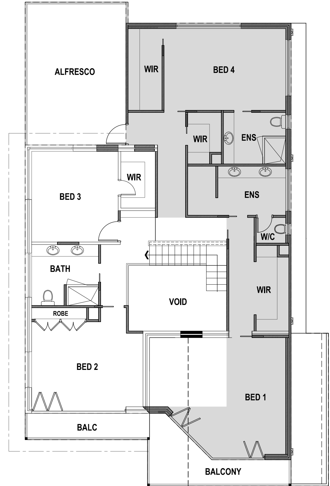
UPPER FLOOR PLAN
